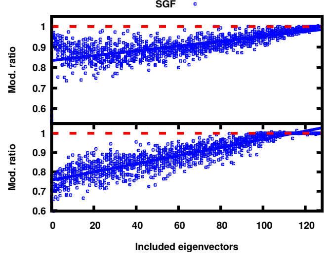
Fig. 6. Modularity ratio for Spectral Graph Forge varying \alpha on our simple graphs with 2 communities (upper plot) and 8 communities (lower plot).
