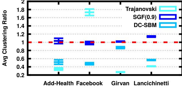
Fig. 10. Means and 99% confidence intervals for average clustering ratio, by data set.
