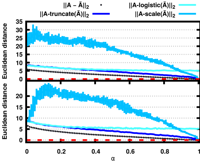
Fig. 4. Baseline and normalized A, \tilde{A} distances for Erdős-Rényi graphs (upper plot) and Barabási-Albert graphs (lower plot), by \alpha . Ideally, normed matrix distances should be close to \|A - \tilde{A}\| .
