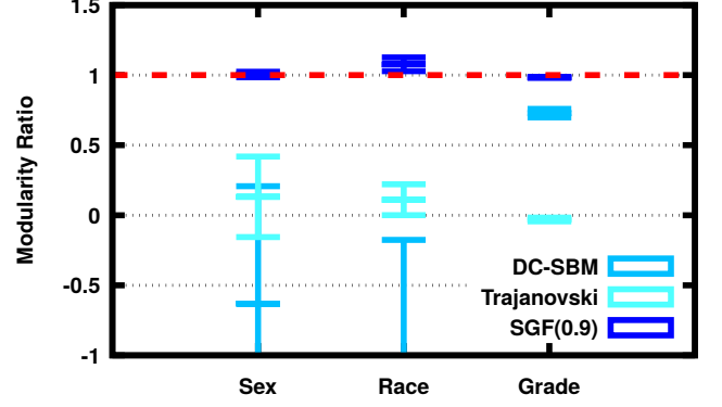
Fig. 12. 99% confidence interval on attribute modularity ratio for the Add-Health dataset.
