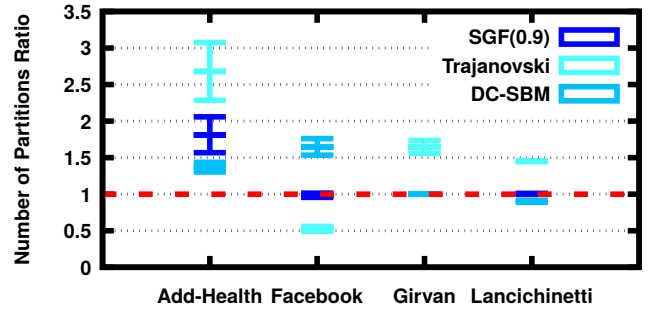
Fig. 9. Means and 99% confidence intervals for the partition number ratio, by data set. Note that the SGF(0.9) and DC-SBM algorithm results overlap with the Girvan data set graphs.
