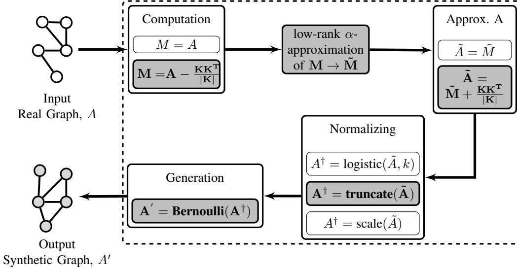
Fig. 2. The pipeline of the Spectral Graph Forge (SGF) Framework. Given an undirected graph adjacency matrix A as input, SGF outputs a “similar” one A' from which we can build the corresponding graph, called SGF( \alpha ). Sub-blocks indicate mutually exclusive options for each step. The focus of this paper is on using SGF to target modularity, by setting M = B = A - (KK^T)/|K| , and the corresponding blocks are highlighted in grey.
