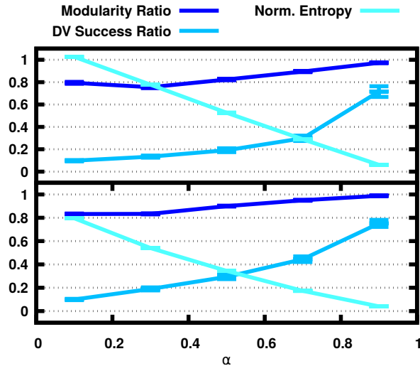
Fig. 13. Means and 99% confidence intervals for graph distribution entropy and DV de-anonymization success rates on one Add-Health graph (upper plot) and one Facebook graph (lower plot), by \alpha .
