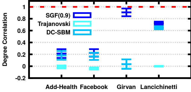
Fig. 11. Means and 99% confidence intervals for degree sequence correlation, by data set. Note that the DC-SBM result lower bound overlaps the Trajanovski results with the Girvan dataset.
