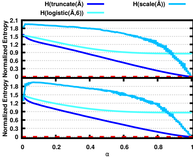
Fig. 5. Entropy of generated graphs using three different normalization functions for Erdős-Rényi input graphs (upper plot) and Barabási-Albert graphs (lower plot) computed for different values of \alpha .
