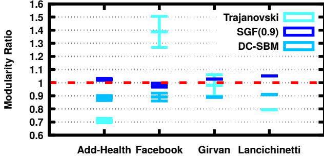
Fig. 8. Means and 99% confidence intervals for the modularity ratio, by method and data set.
