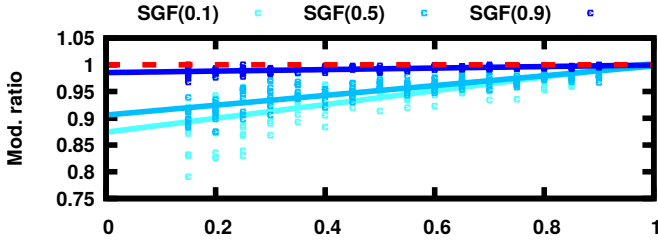
Fig. 7. Modularity ratio for Spectral Graph Forge on our simple graphs varying their connectivity with 2 communities.
