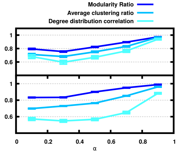
Fig. 14. Means and 99% confidence intervals for degree distribution correlation and average clustering ratio on one Add-Health graph (upper plot) and one Facebook graph (lower plot), by \alpha .
